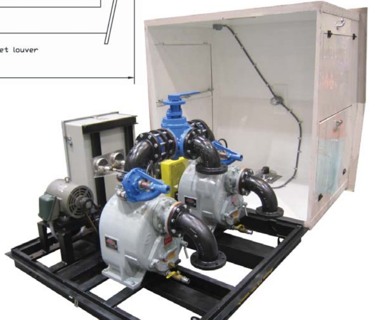
S-4 Duplex Pump Station open for heavy maintenance
