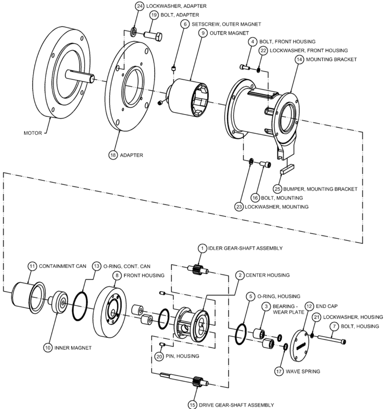
Exploded View Drawing – 2-Series Mini Pump
