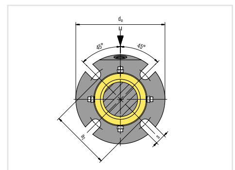
Seal cover
