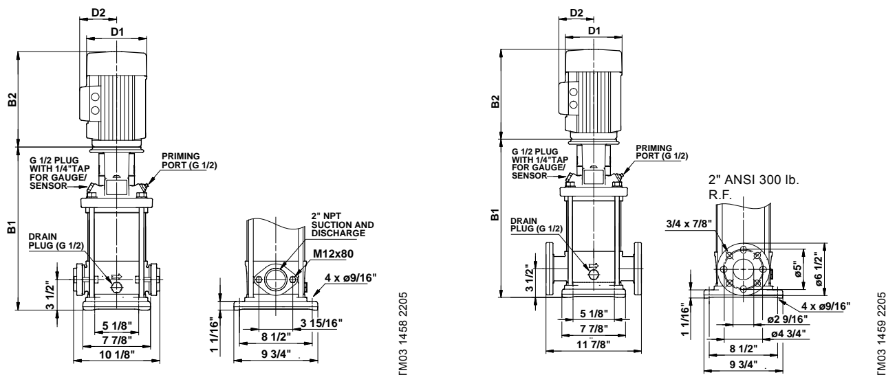
ANSI dimensions [inch (mm)]
