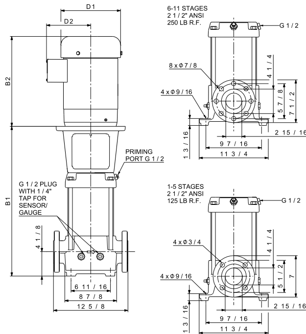
ANSI dimensions [inch (mm)]
