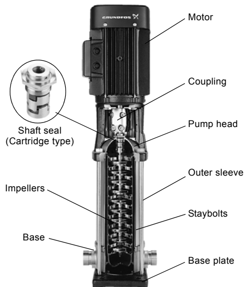
Fig. 2 CR pump
