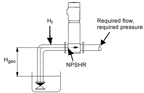
Fig. 9 Sizing data
