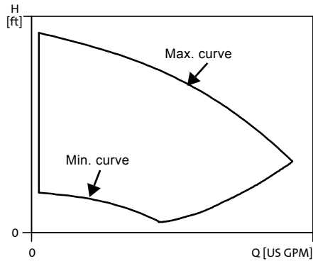
Fig. 12 Min. and max. performance curves
