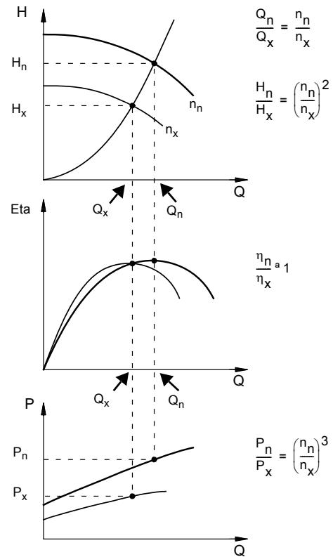
Fig. 13 Affinity equations
