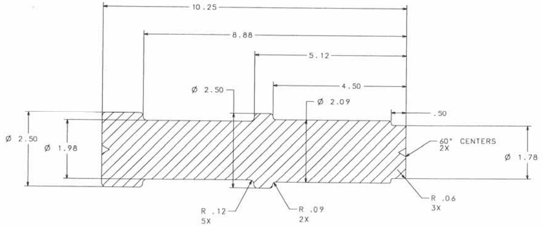
CFR / ETFE Drive Lug Disassembly Tool (PT0820) Material: UHMW Fig. 11-8
