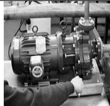
Fig. 7-4: Unbolt Bracket from Rear Support
