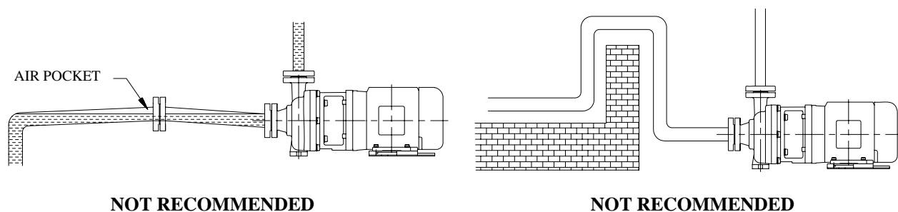
Fig. 5-1: Pump Installations
