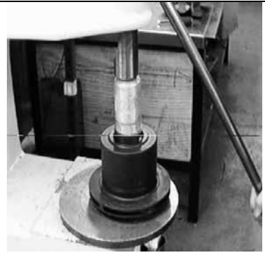
Fig.8-5: Insert Bushing into Impeller with Arbor Press
