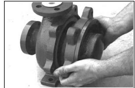
Fig. 8-9: Fit Casings Together
