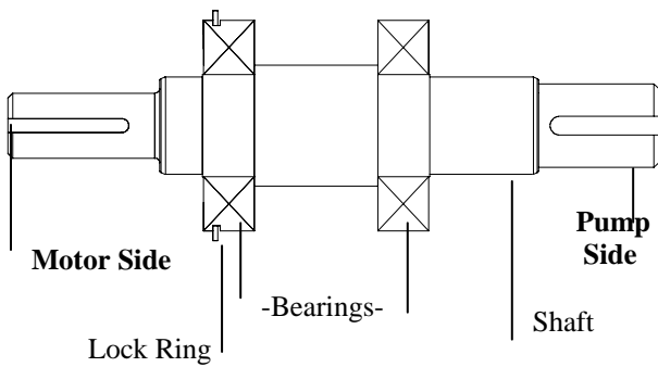
Fig. 12-18: Shaft Assembly
