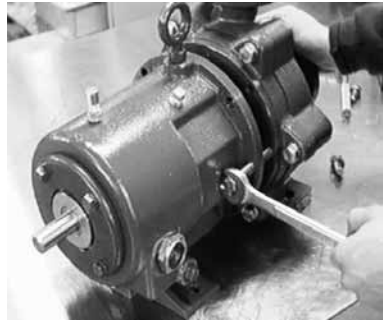
Fig. 12-4: Jackscrews to Decouple Drives
