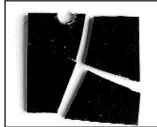
XLPE exposed 6 months in 98% H 2 SO 4 3.4 ft. pounds @ -40° F.
